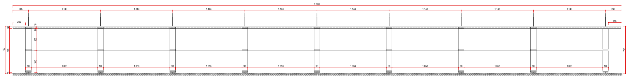
VISTA FRONTAL
